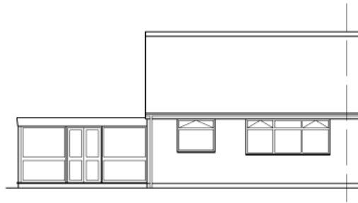
REAR ELEVATION
