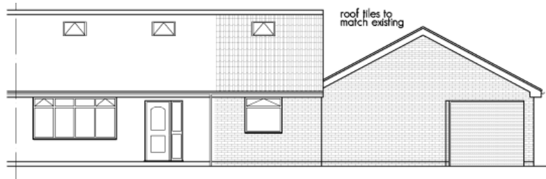
FRONT ELEVATION
